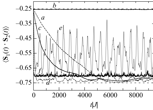
Fig.3 (color online). Time evolution of the correlation \langle \Psi(t) | \mathbf{S}_1 \cdot \mathbf{S}_2 | \Psi(t) \rangle of the two spins in the central system. Environment containing N = 16 quantum spins. Dashed horizontal line at -1/4 : Correlation in the initial state ( \langle \Psi(t=0) | \mathbf{S}_1 \cdot \mathbf{S}_2 | \Psi(t=0) \rangle = -1/4 ); Horizontal line at -3/4 : Correlation in the singlet state. For all curves (a – f) \Delta_{i,j}^{(x)} = \Delta_{i,j}^{(y)} = 0 , that is H_{\text{int}} is Ising like. The values of \Delta_{i,j}^{(z)} are: (a) random -0.0375 |J| or 0.0375 |J| , (b – e) random -0.075 |J| or 0.075 |J| , (f) random -0.15 |J| or 0.15 |J| . The values of \Omega_{i,j}^{(\alpha)} are uniform random numbers in the range: (b) [-0.0375 |J|, 0.0375 |J|] , (a, c) [-0.15 |J|, 0.15 |J|] , (d, f) [-0.3 |J|, 0.3 |J|] and (e) [-|J|, |J|]
