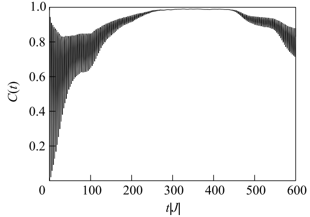
Fig.2 (color online). Time evolution of the concurrence C(t) for the case of a frustrated antiferromagnetic environment. The interactions of the central system and the environment are uniform random numbers in the range -0.15|J| \leq \Delta_{i,j}^{(\alpha)} \leq -0.05|J| . The environment contains 14 quantum spins, arranged on a triangular lattice and interacting with nearest neighbors only. The nonzero exchange integrals are uniform random numbers in the range -0.55|J| \leq \Omega_{i,j}^{(\alpha)} \leq -0.45|J| . The transition from an unentangled state ( C(t) = 0 ) to a nearly fully entangled state ( C(t) = 1 ) is evident, as is the onset of recurrent behavior due to the finite size of the environment
