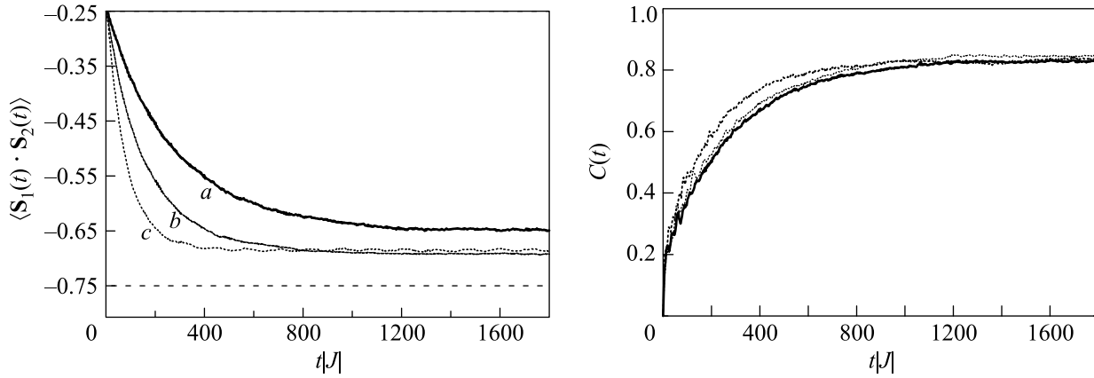
Fig.1 (color online). Left: Time evolution of the correlation \langle \Psi(t) | \mathbf{S}_1 \cdot \mathbf{S}_2 | \Psi(t) \rangle of the two spins in the central system. Dashed horizontal line at -1/4 : Correlation in the initial state ( \langle \Psi(t=0) | \mathbf{S}_1 \cdot \mathbf{S}_2 | \Psi(t=0) \rangle = -1/4 ); Horizontal line at -3/4 : Expectation value in the singlet state; (a) Environment containing N = 14 quantum spins; (b) N = 16 ; (c) N = 18 . The parameters \Omega_{i,j}^{(\alpha)} and \Delta_{i,j}^{(\alpha)} are uniform random numbers in the range [-0.15|J|, 0.15|J|] . Right: Time evolution of the concurrence C(t) for three different random realizations of a spin glass environment. The parameters are uniform random numbers in the range -0.15|J| \leq \Omega_{i,j}^{(\alpha)}, \Delta_{i,j}^{(\alpha)} \leq 0.15|J| and the environment contains N = 14 quantum spins. The transition from an unentangled state ( C(t) = 0 ) to a nearly fully entangled state ( C(t) = 1 ) is clearly seen
