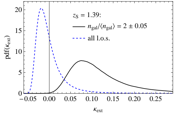
FIG. 4.— Probability distribution for the external convergence \kappa_{\text{ext}} obtained from combining results of galaxy number counts around B1608+656 with results from ray-tracing through the Millennium Simulation. Compared are the distribution along lines of sight with a relative galaxy number density n_{\text{gal}}/\langle n_{\text{gal}} \rangle = 2.00 \pm 0.05 (solid line) to the distribution along all lines of sight (dotted line).
