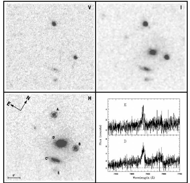
FIG. 2.— HST images of MG 2016+112: WFPC2 F555W ( V ) and F814W ( I ) images and the NICMOS-2 F160W ( H ) image. The exposure times are 5200 s ( V and I ) and 5120 s ( H ), and the pixel scales are 0''.0455 ( V ), 0''.1 ( I ), and 0''.075 ( H ). The two lensed quasar images (A and B), the primary lens galaxy (D), the arc C', and the additional galaxy (E) are indicated on the H -band image. The emission from the [O II] doublet detected from galaxies E and D is shown in the bottom right panel. Note that the doublet in D is blended by the large velocity dispersion.
