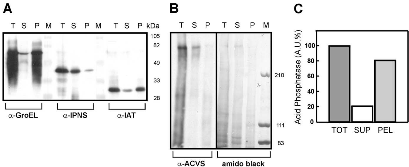
Fig. 2. Subcellular fractionation and sedimentation of organelles. Analysis of proteins present in the post-nuclear supernatant fraction of disrupted protoplasts (T) of P. chrysogenum DS04825. After centrifugation at 100,000g, the cytoplasmic material was recovered in the supernatant (S) fraction whereas organellar and membranous material was pelleted (P) and resuspended to the same volume as the original total extract. For comparison, aliquots of identical volume of the three fractions were loaded on the SDS-PAGE. Markers (M) are indicated. (A) Western analysis after 12% SDS-PAGE using antibodies against IPNS, AT, and E. coli GroEL. (B) Western analysis after 5% SDS-PAGE using an anti-ACV synthetase antibody. As a control, the blot was stained with amido black showing intact enzyme as a high molecular mass protein. (C) Activity of the vacuolar marker acid phosphatase in the different fractions.
