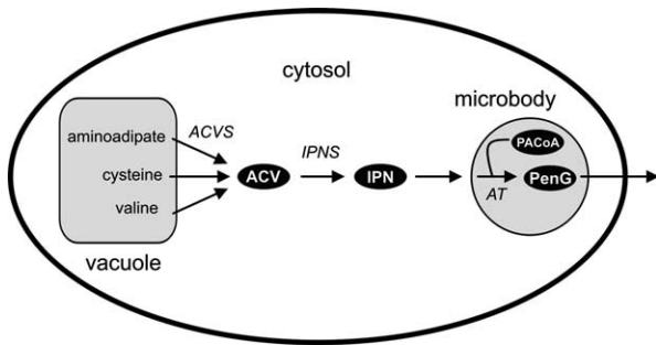
Fig. 4. Scheme for the compartmentalization of penicillin biosynthesis in P. chrysogenum . ACVS, ACV synthetase; ACV, \delta -L- \alpha -aminoadipyl-L-cysteiny-D-valine; AT, acyltransferase; IPNS, IPN synthase; IPN, isopenicillin N; PACoA, phenylacetyl-Coenzyme A; PenG, penicillin G.
