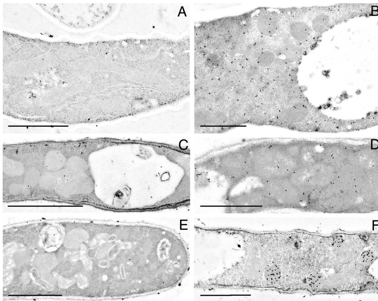
Fig. 3. Immuno-gold labeling of ACV synthetase (A and B), IPN synthase (C and D) and acyltransferase (E and F) in electron micrographs of mycelium of P. chrysogenum . For immuno-localization, strain Wis54-1255 was used (B, D, and F), and the npe10 (A and C) or npe6 , an acyltransferase mutant (E). The strains were grown under penicillin producing conditions. Labeling experiments were carried out as described in the text. The drawn marker represents 1 \mu\text{m} . M, mitochondrion; V, vacuole.
