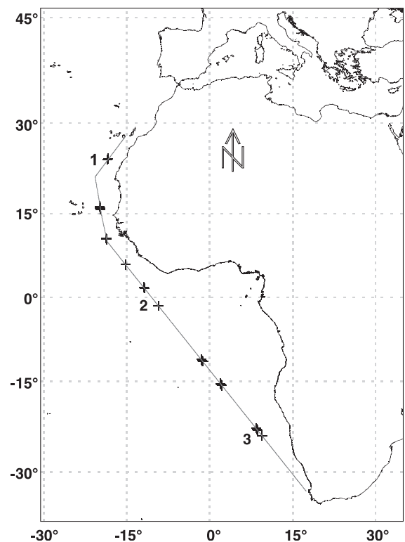
Fig. 1. Cruise track of cruise ANT18/1 of RV 'Polarstern' from Bremerhaven (Germany) to Cape Town (South Africa). The positions of H_2O_2 measurements are indicated by crosses, the positions of the experiments by numbers.
