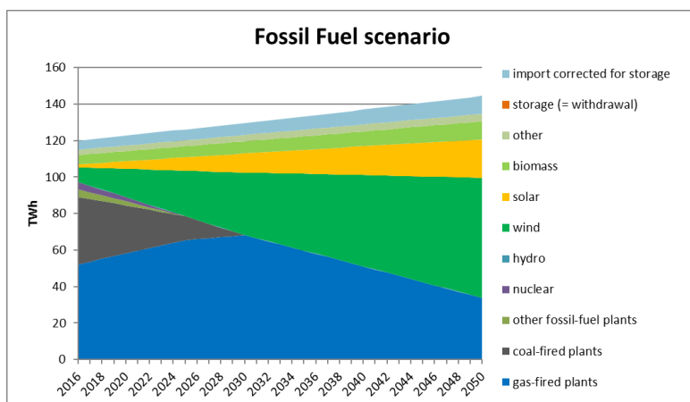
Figure 6.1: Supply of electricity, per scenario, 2016-2050
