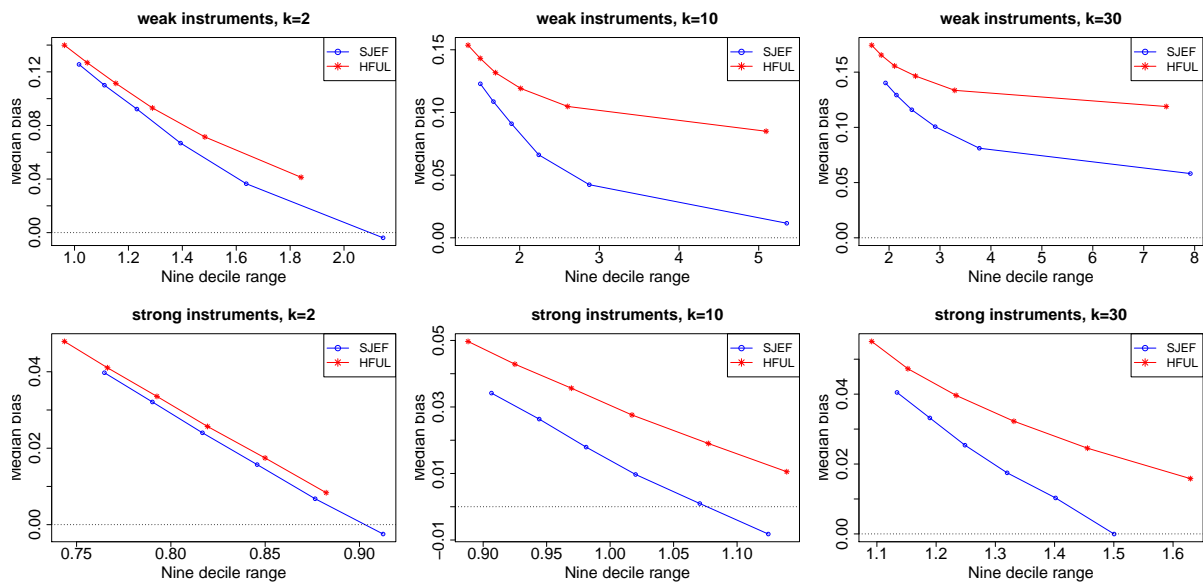
Figure 2: R_{\varepsilon^2|z}^2 = 0.2 : Median bias against the Nine decimal range of HFUL with c = 0, 1, 2, 3, 4, 5 from right to left, and SJEF for \alpha = 0, 1, 2, 3, 4, 5 from right to left, based on 20,000 replications.
