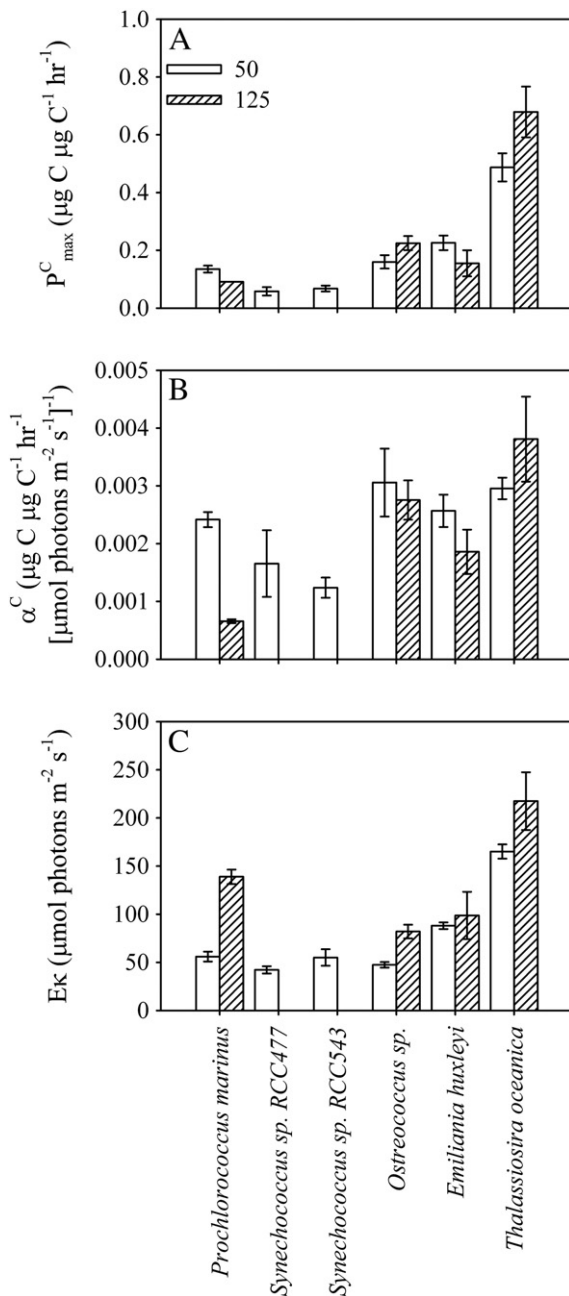
Fig. 6. Averages ( \pm standard deviation, n=4 ) for the maximum photosynthetic rate (A), initial rate of photosynthesis (B), and photoadaptation index (C) normalized to carbon of the six phytoplankton strains at 50 and 125 \mu\text{mol photons m}^{-2} \text{s}^{-1} . Values for constant and dynamic irradiance treatments were grouped according to the average irradiance given during the treatment (50 or 125 \mu\text{mol photons m}^{-2} \text{s}^{-1} ).
