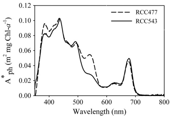
Fig. 4. Example of the specific absorption coefficient \alpha^*_{ph} for Synechococcus sp. RCC477 and RCC543 at 50 \mu\text{mol photons m}^{-2} \text{s}^{-1} . Differences in phycobilisome pigmentation are clearly visible around 550 nm.
