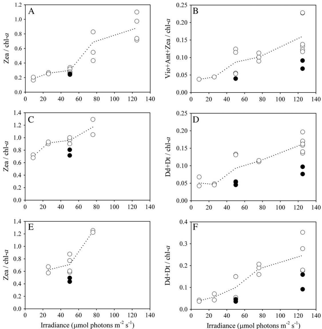
Fig. 3. Photoprotective pigments to chlorophyll a ratio for (A) Prochlorococcus marinus , (B) Ostreococcus sp., (C) Synechococcus sp. RCC477, (D) Emiliania huxleyi , (E) Synechococcus sp. RCC543, and (F) Thalassiosira oceanica at the different irradiances of the constant (open circles) and dynamic (filled circles) irradiance regimes. Abbreviations: Chl- a : chlorophyll a , Vio: violaxanthin, Ant: antheraxanthin, Zea: zeaxanthin, Dd: diadinoxanthin, and Dt: diatoxanthin.
