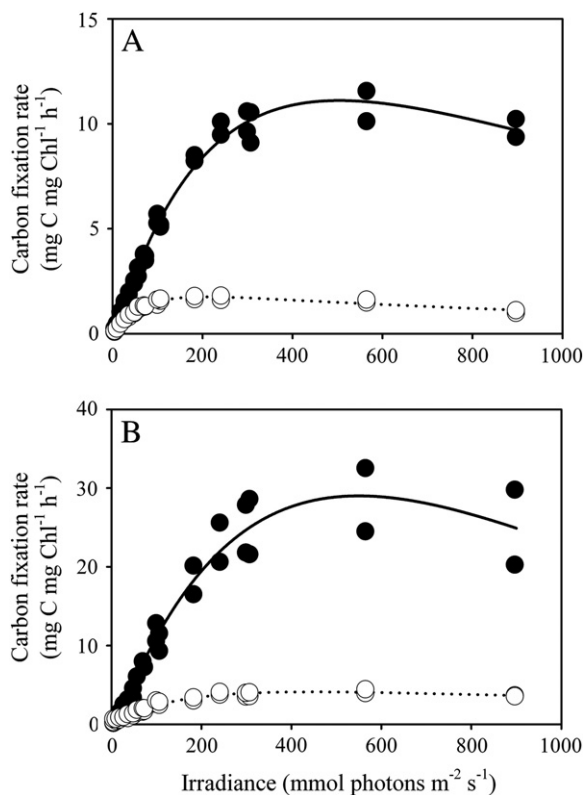
Fig. 5. Photosynthesis versus irradiance curves for Prochlorococcus marinus (open circles) and Thalassiosira oceanica (filled circles) for the (A) 50 and (B) 125 \mu\text{mol photons m}^{-2} \text{ s}^{-1} constant irradiance treatments. The average fit is given ( n = 2 ). Note that the scales of the carbon fixation rates are different between the figures.
