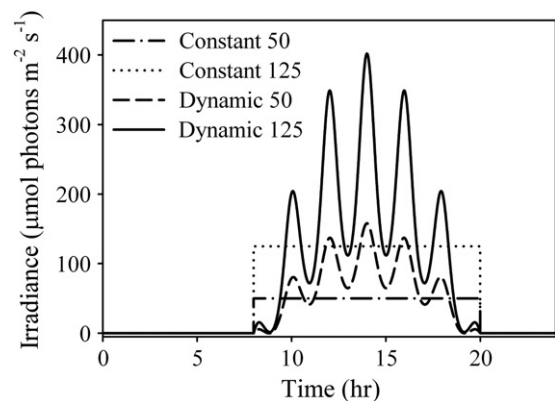
Fig. 1. Constant and dynamic irradiance regimes, averaging at 50 and 125 \mu\text{mol photons m}^{-2} \text{s}^{-1} .
