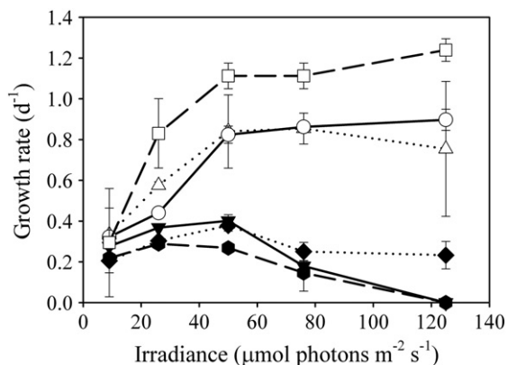
Fig. 2. Average growth rates ( \pm standard deviation, n \geq 2 ) for Prochlorococcus marinus (filled diamonds), Synechococcus sp. RCC477 (filled triangles), Synechococcus sp. RCC543 (filled octagons), Ostreococcus sp. (open triangles), Emiliania huxleyi (open circles), and Thalassiosira oceanica (open squares). Negative values in Synechococcus sp. (both strains) at 125 \mu\text{mol photons m}^{-2} \text{s}^{-1} were set to zero.
