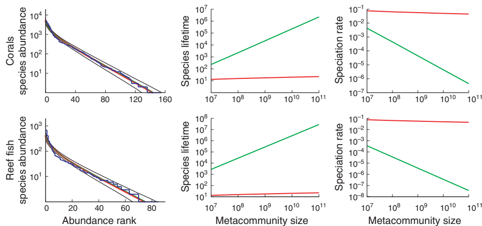
Figure 4 Top left panel: a fit to coral reef metacommunity data (shown in blue) using the standard point mutation model with \theta=19.85 (red) and protracted speciation model with \theta=20.13 and \tau'=2.23\times 10^{-6} (green). These parameters represent the global optimum in parameter space calculated with eqn 4. The two black lines represent 1 SD on either side of the mean prediction under protracted speciation, produced by analysing 4 000 000 simulations of the model (using algorithms described in Appendix S1). It can clearly be seen that both models fit the abundance data equally well: we increased the thickness of the red line otherwise it would be completely hidden behind the green line. The top centre and top right panels show the species lifetimes (in generations) and speciation rates (per species per generation), respectively, and were plotted using the same parameter values as those used for the top left panel. The lower set of panels show the same results for a reef fish metacommunity sample for which the best fitting \theta was 15.82 under point mutation (red) and \theta=16.21 , \tau'=3.77\times 10^{-5} under protracted speciation (green).
