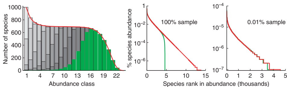
Figure 3 Species abundance distributions (SADs) for the log-series and difference log-series (DLS). Left panel: histogram of numbers of species in each abundance class for J_M = 10^9 and \mu = 0.000001 predicted by the log-series distribution (red line) and the DLS with a variety of different transition times \tau = 0, 1, 10, 100, 1000, 10\ 000 (bars with darker colours corresponding to larger \tau and \tau = 10\ 000 in green). The j th abundance class is defined as containing species with j \leq abundance < 2j . As \tau increases, there are dramatically fewer rare species, but the more abundant species follow the log-series distribution very closely. The remaining panels show the same data for the log-series (red line) and DLS with \tau = 10\ 000 (green line) as a plot of log abundance vs. rank in abundance. The whole metacommunity is shown in the centre, where the DLS is clearly distinct from the log-series. A random sample of 0.01% of individuals is plotted on the right showing that after sampling it is nearly impossible to observe the difference between the DLS and log-series.
