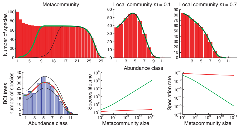
Figure 5 Local community species abundances compared with the regional species abundances and empirical data. Top left panel: a metacommunity abundance distribution with J_M=10^{10} , \theta=100 under different modes of speciation. Point mutation speciation (red bars), protracted speciation with \tau=100 (green line) protracted speciation with \tau=10\,000 (black line). Top centre and right panels show dispersal limited local community samples m=0.1 (top centre) and m=0.7 (top right) for all three metacommunities. It is clear that in these local community samples we no longer see the very significant differences in the metacommunities from which they are drawn. A fit to locally sampled species local community abundance data for trees on BCI (Condit 1998; Hubbell et al. 1999, 2005) is shown in the bottom left panel. The parameters used were \theta=47.67 and m=0.093 for point mutation (red) and \theta=47.96 , \tau'=8.15\times 10^{-8} and m=0.093 for protracted speciation (green). Blue bars show empirical data and the two black lines represent the 1 SD on either side of the mean of the protracted speciation result, calculated by simulation as in Fig. 4. The bottom centre and bottom right panels show speciation rate and species lifetime for the same optimal parameters as used to fit the species abundances in the bottom left panel.
