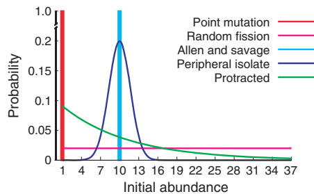
Figure 2 The probability distributions of initial abundances of new species under various speciation mechanisms. In point mutation speciation and the alternative of fixed initial abundances proposed by Allen & Savage (2007), each new species begins with a fixed abundance. In random fission a population is randomly cleaved in two with the smaller part forming a new species leading to a constant probability for all possible initial abundances up to a size half that of the parent population. Peripheral isolate speciation yields a normal distribution with both mean and variance as model parameters and so it reduces to the case of fixed initial abundance (Allen & Savage 2007) when the variance is set to zero. The only mechanistically derived distribution here is that of protracted speciation where initial abundances follow the distribution given in eqn 8.
