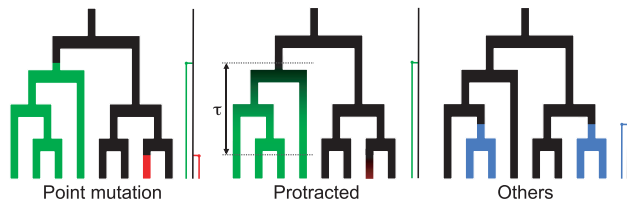
Figure 1 A simple example genealogy for various possible modes of speciation with different colours denoting different species. The left panel shows the point mutation speciation case where new species arrive as singletons. The centre panel shows protracted speciation where instead of appearing instantaneously, new species gradually evolve over a period of time \tau shown with the colour of one species gradually fading into the colour of the next. Individuals belonging to an ‘incipient’ species (e.g. shades of dark green) would not be recognized as being a novel species and are classified as natural variants of the parent species shown in solid black, after the transition time a new species (solid green) is clearly recognized. The far right panel shows peripheral isolate speciation, random fission speciation and the case where initial abundances are fixed but greater than one. In each case we show the phylogeny of good species just to the right of the genealogy. Splits in the phylogeny correspond to speciation events that have had time to complete.
