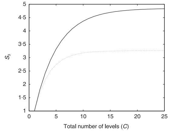
Fig. 2. Dependence of the quantity S_3 = \sum_{k=1}^C [1/(N_k)^{\frac{1}{3}}] on the total number of levels, C , for two networks. Solid curve: a network where at each node the number of vessels doubles ( v_k = 2 for all k ). Dotted curve: a network where at each node the number of vessels triples ( v_k = 3 for all k ). Note the small linear scale at the y-axis which implies that even for small C the dependence of S_3 on C and hence on M is negligible.
